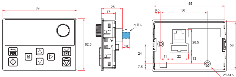
图8-14 HWF750-JP-LED-BD外引+本机操作面板尺寸
